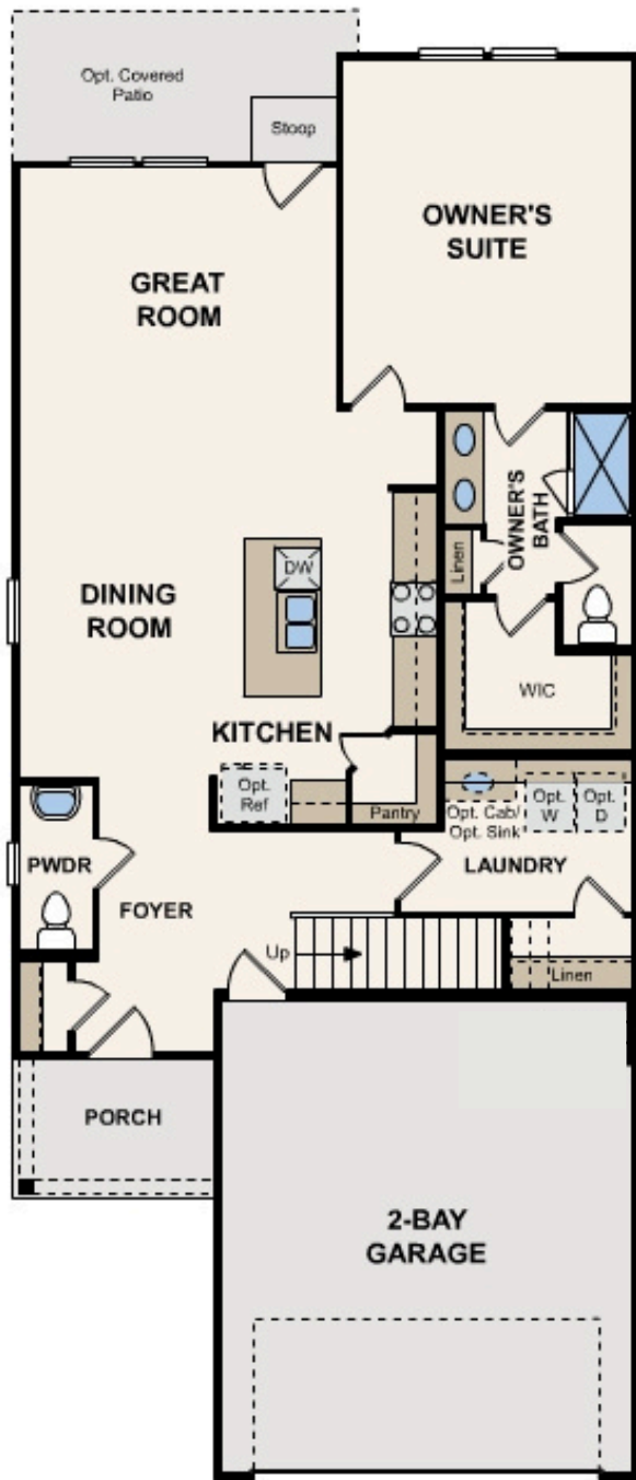
FIRST FLOOR
